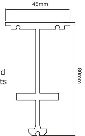
TRACK SECTION
